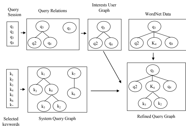
Figure 3: The refined query graph generation process.
