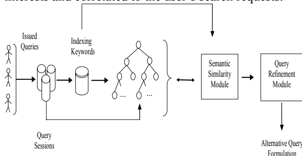
Figure 2: The query refinement process.
